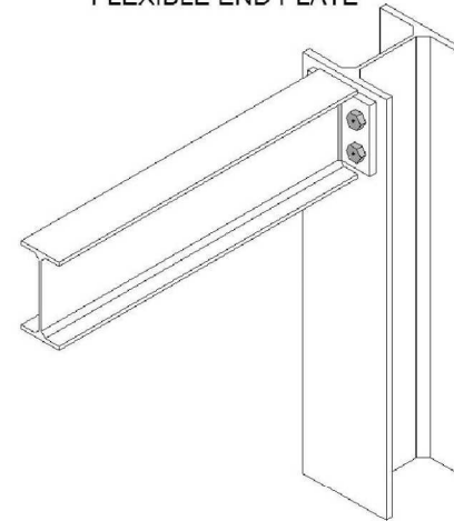
SINGLE-SIDED BEAM TO COLUMN (FLANGE)
