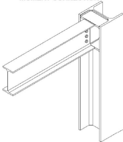
SINGLE-SIDED BEAM TO COLUMN (WEB)
