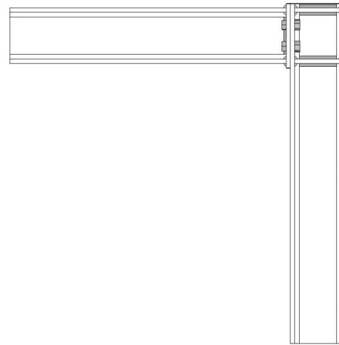
MOMENT CONNECTION
