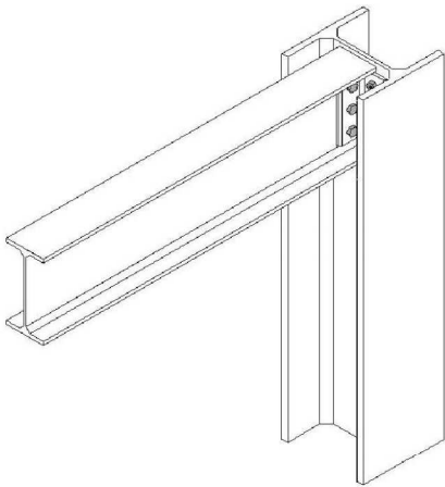
SINGLE-SIDED BEAM TO COLUMN (WEB)
